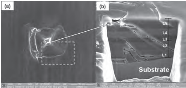
Figure 5: (a) Top view SEM of 5N Vickers indent, (b) Cross-section SEM of indented area after FIB.
