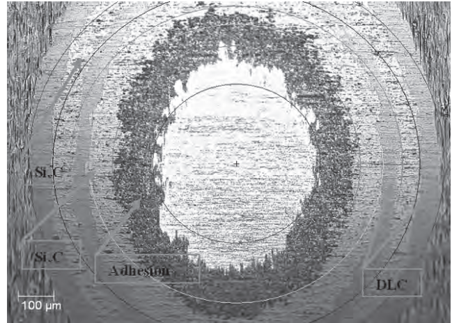
Figure 3: Optical micrograph of a Calotest crater showing multilayer coating structure.
