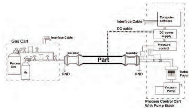
Figure 1: Diagram of Process Set-up [8].
