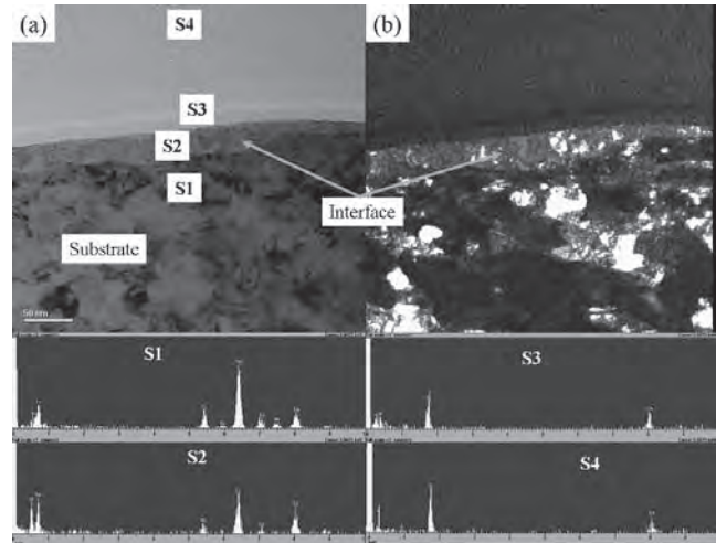
Figure 4: (a) Bright field and (b) dark field TEM micrographs and associated EDX spectra showing substrate-coating interface.
