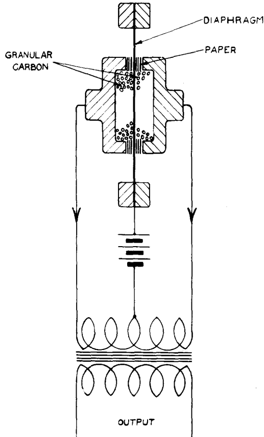
Fig. 2. Diagram of connections between double button type of microphone and amplifier.
