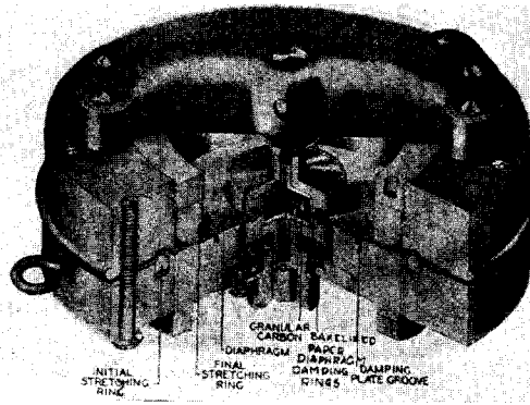
Fig. 1. Carbon broadcasting transmitter.
