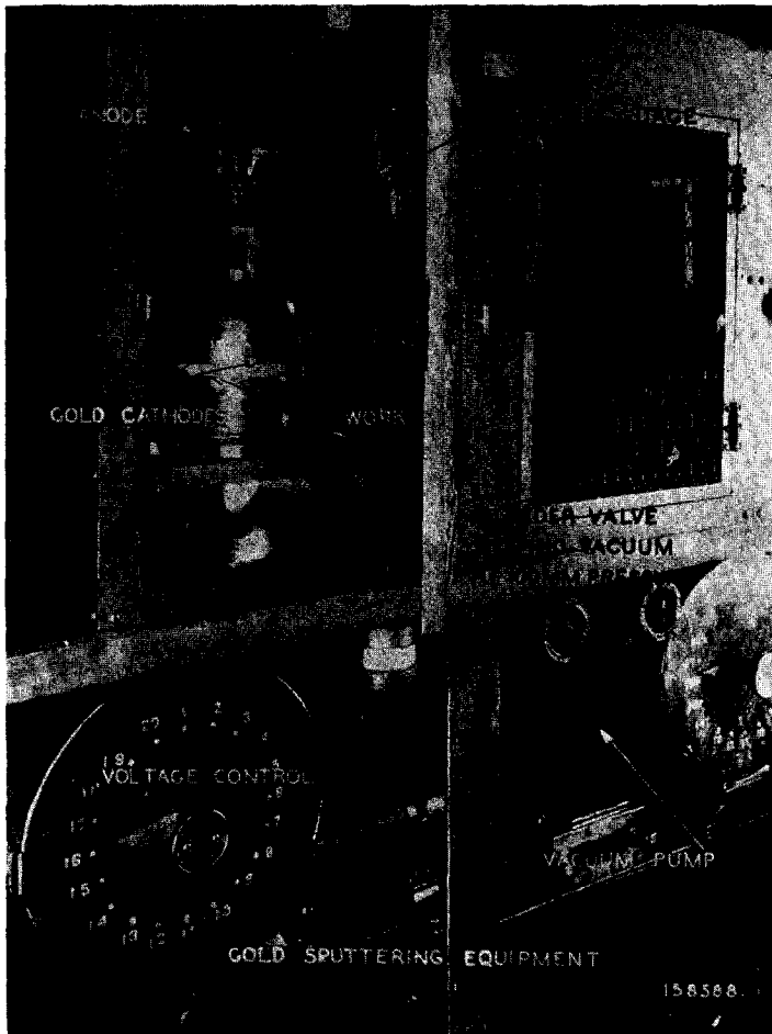
Fig. 3. Commercial sputtering unit.
