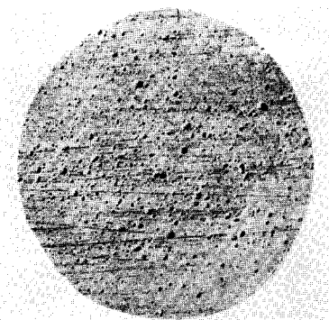
Fig. 6a. Representative gold plated diaphragm surface after 3 months service showing blisters.
